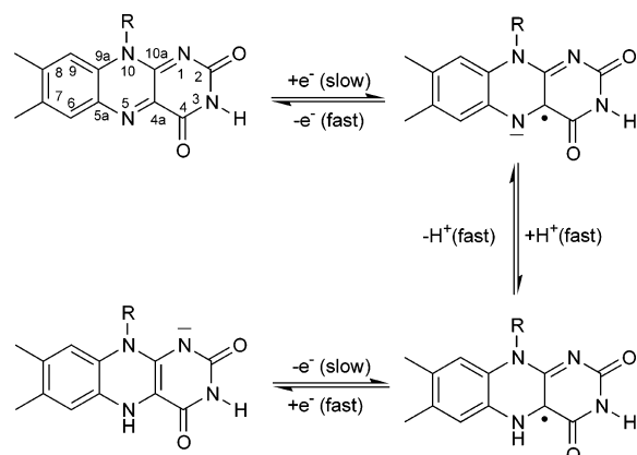
Scheme 1. Flavin Numbering and Common Oxidation/Protonation States Observed for the Flavin Cofactor
