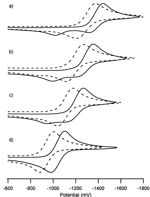
Figure 2. Cyclic voltammograms of selected 7,8-substituted flavins vs ferrocene, CH 2 Cl 2 , 23 °C, 0.1 M TBAP used as electrolyte. The solid lines indicate each flavin free in solution (5 mM), the dashed lines are the same flavins in the presence of DAP (50 mM). (a) 1j , (b) 1h , (c) 1d , (d) 1b .
