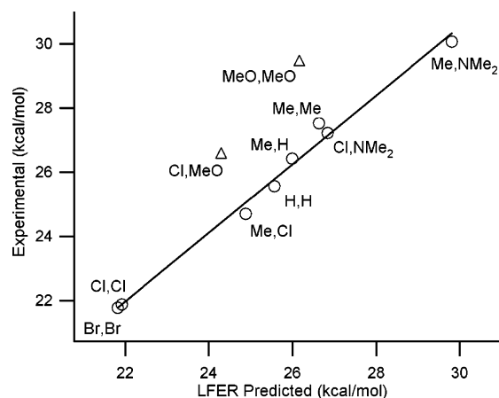
Figure 6. Plot showing correlation between experimental and linear free energy derived values for the reduction potentials of flavins in methylene chloride in the presence of DAP. Slope = 1.07 (methoxy-substituted flavins not included), r^2 = 0.9884 .
