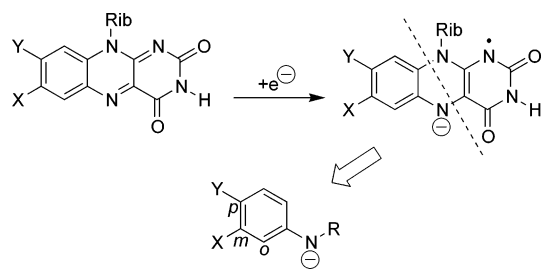
Figure 3. Simplification of the flavin radical anion into a pseudo-phenyl system.
