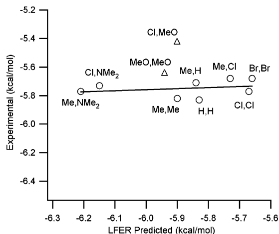
Figure 8. Plot showing the lack of correlation between experimental and linear free energy-derived values for the DAP binding of flavins in the reduced form.
