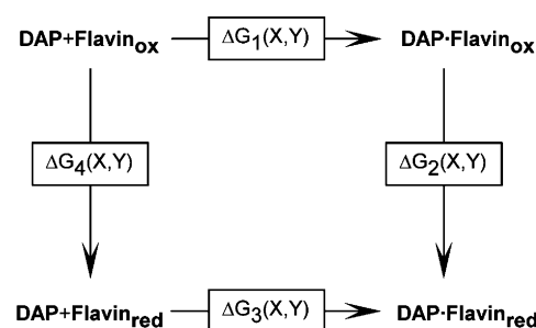
Figure 7. Thermodynamic cycle showing the relationship between the flavin–DAP binding and reduction processes.
